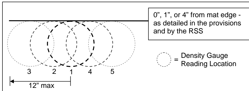
Figure 2: Asphalt density gauge reading pattern less than 6" from mat
