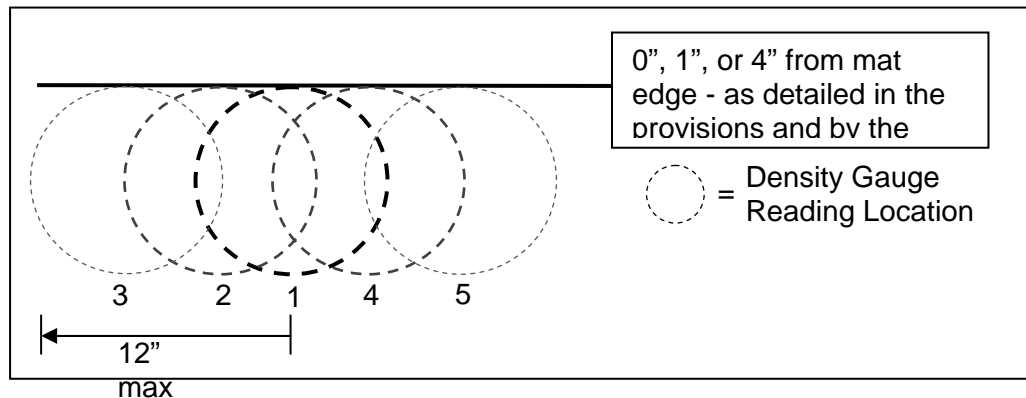
Figure 2: Asphalt density gauge reading pattern less than 6" from mat
